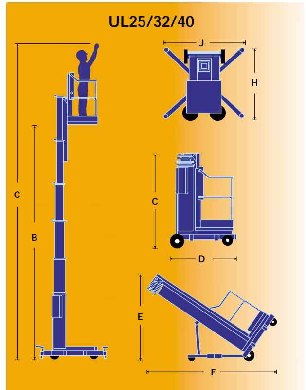
UI 25/32/40 models are fitted with the EZ loader system to assist loading onto pickup trucks.
